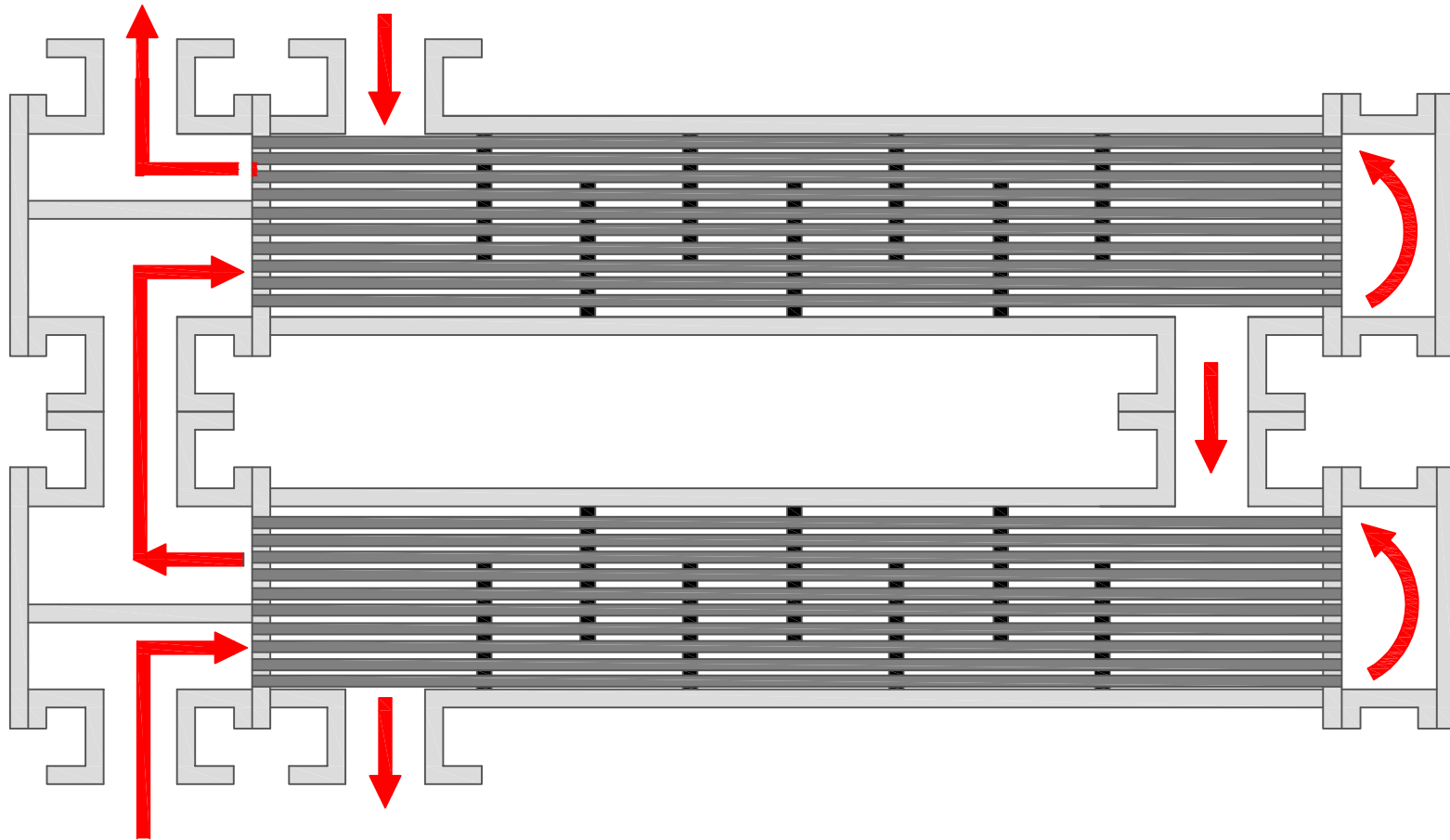
Flow arrangement for two heat exchangers in series
